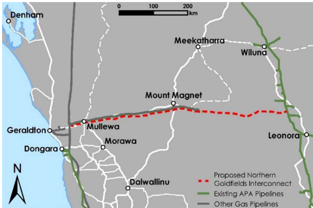
Western Australia Northern Goldfields Interconnect map
