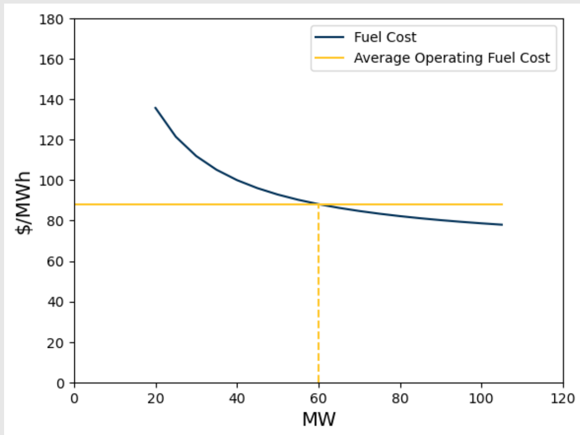
Figure 33. Estimation of Average Operating Cost of Fuel for a stylised fuel cost curve for a generator with increasing thermal efficiency.
