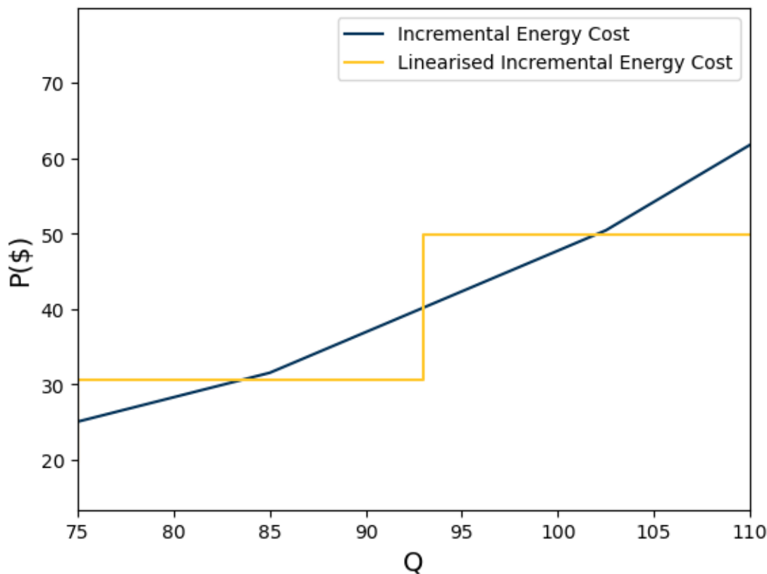
Figure 11. Conversion of Incremental Efficient Variable Cost curve to two-step Price-Quantity Pair
