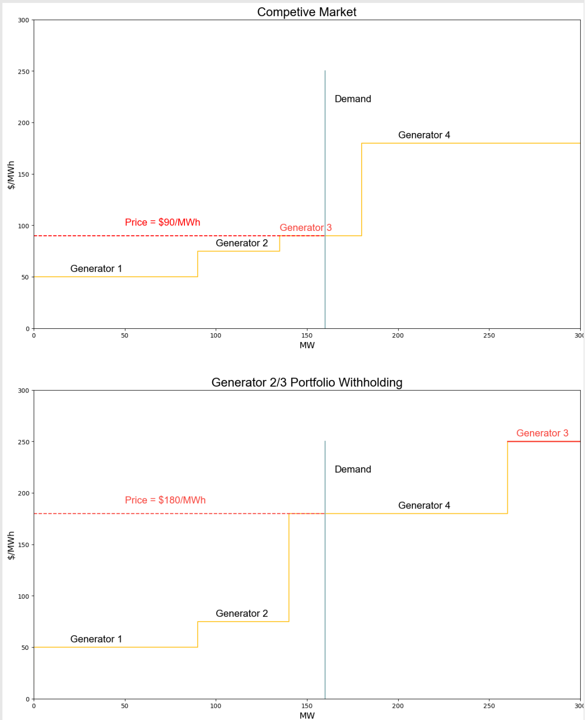
Figure 66. Generator 3 economic withholding
