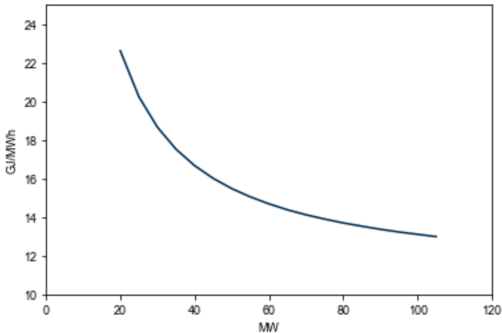
Figure 22. Stylised average heat rate chart for a thermal generator with increasing efficiency
