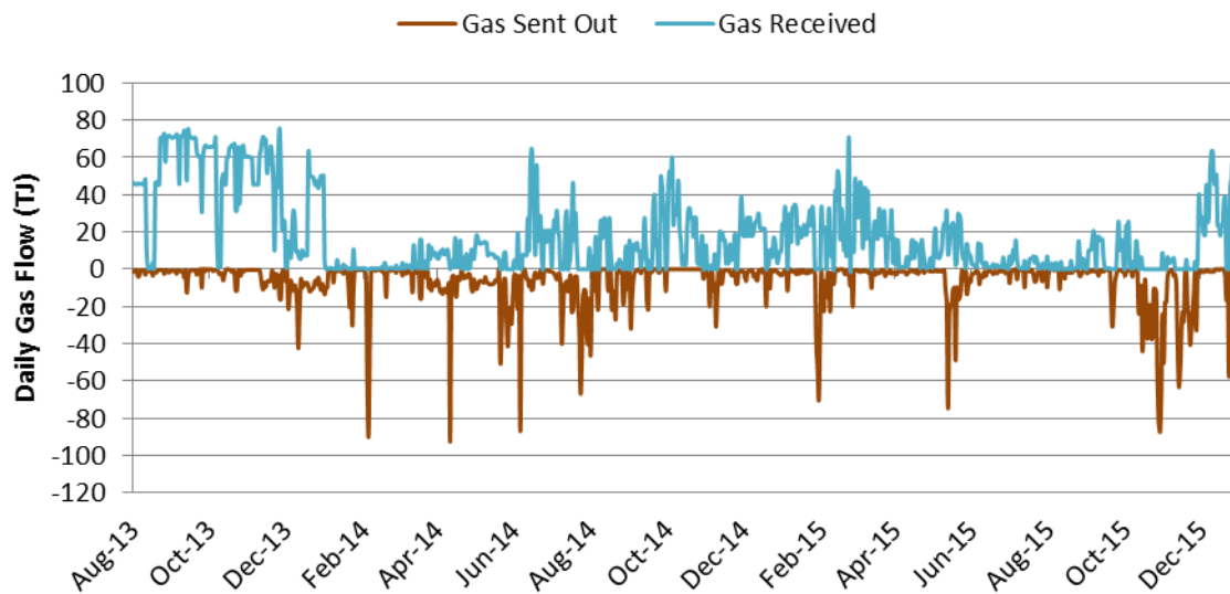
Figure C- 2 Mondarra Gas Storage Facility Operations, Aug 2013 to Dec 2015
