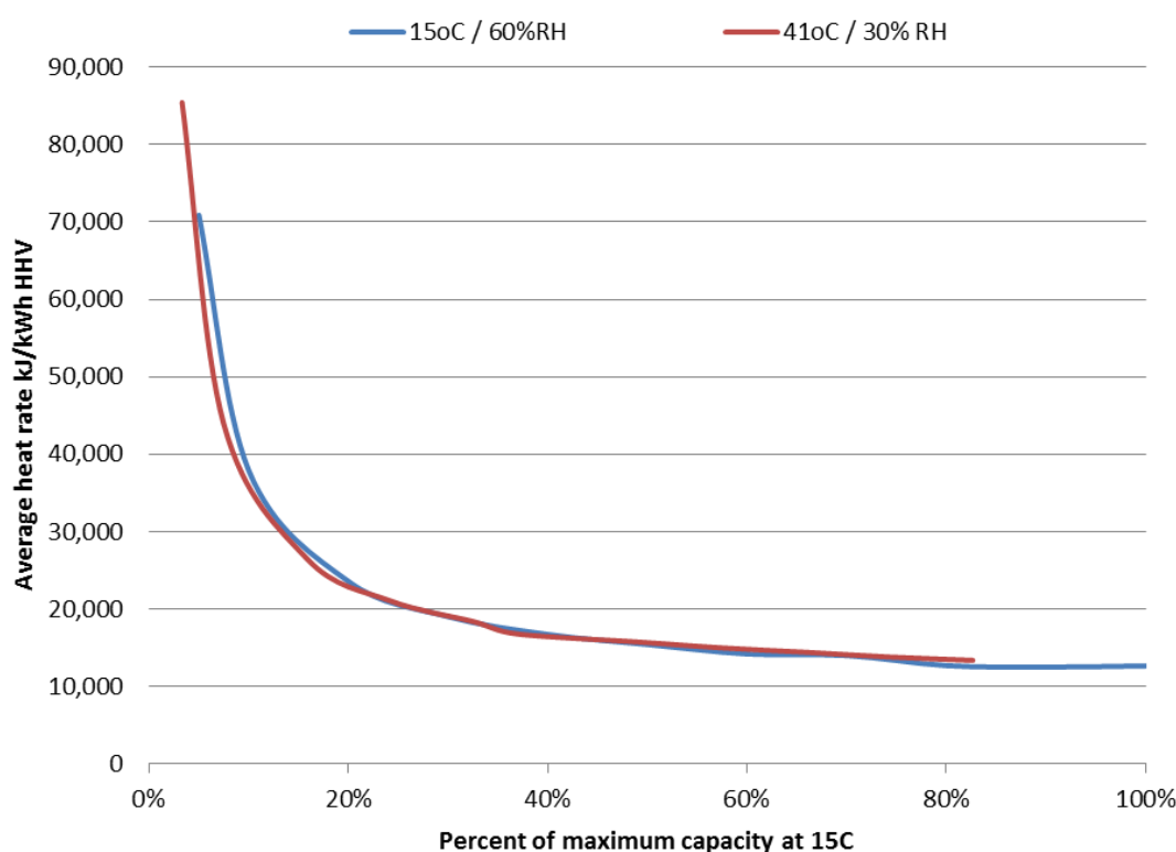
Figure 7 Run-up Heat rate curve for industrial gas turbine (new and clean)
