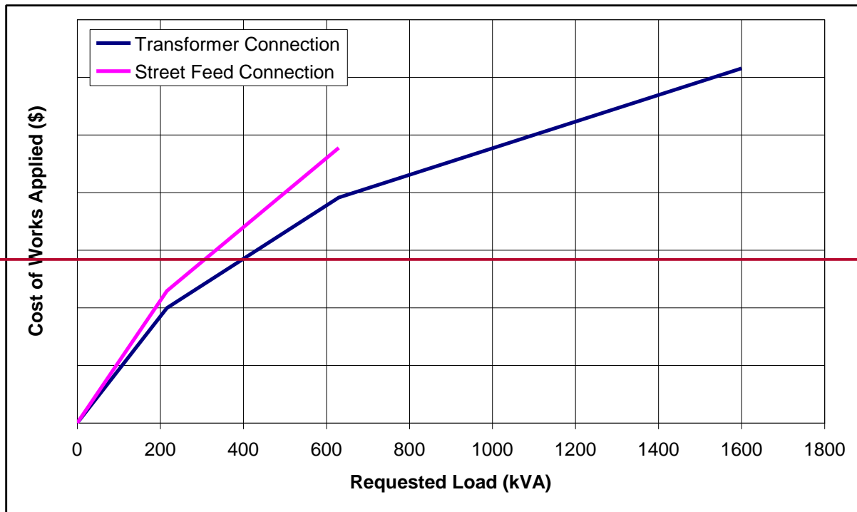
Figure 5.1 – Modelling of the cost of works applied to the customer for Transformer Connections and Street Feed Low Voltage Street Network Connections.
