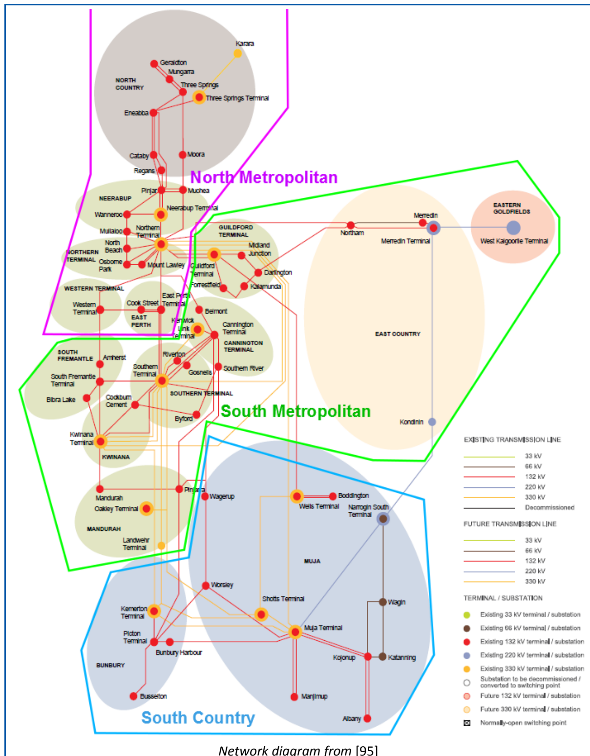
Figure 12.7 – WEM system restart sub-networks
