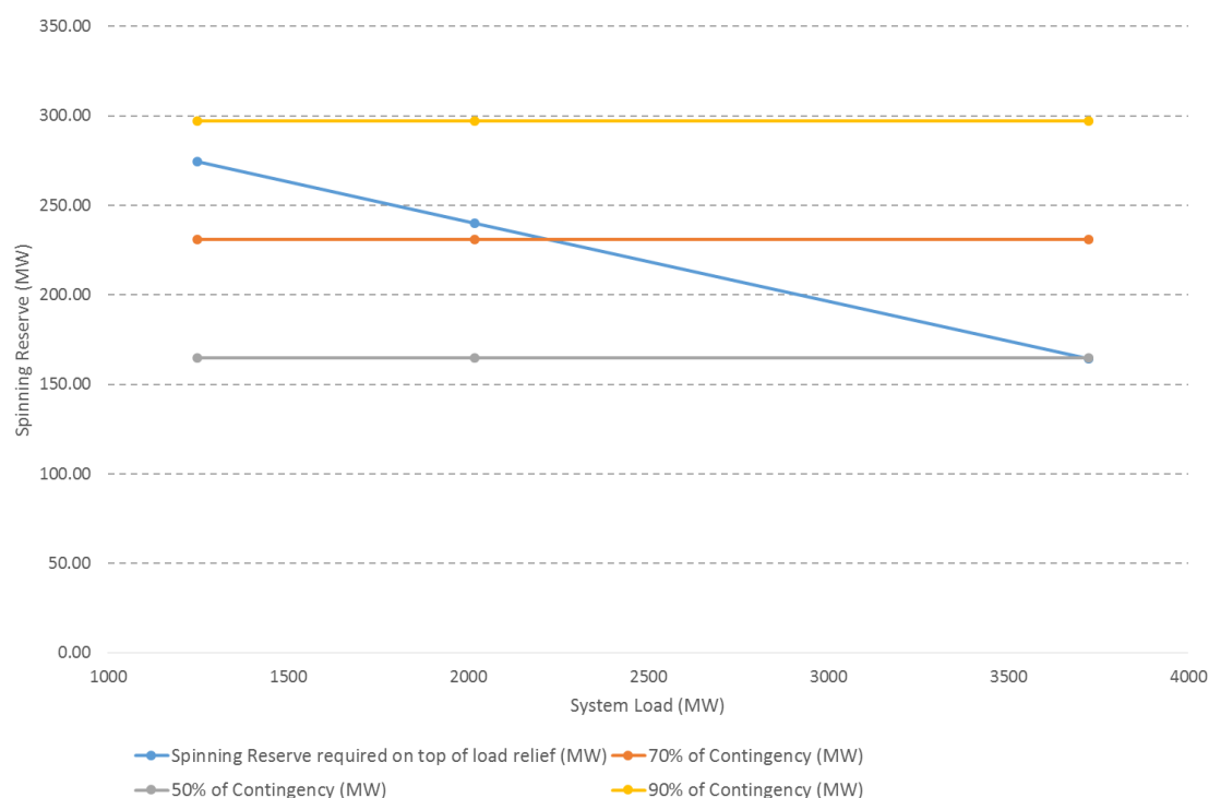
Figure 10.10 – Calculated Spinning Reserve Service requirements
