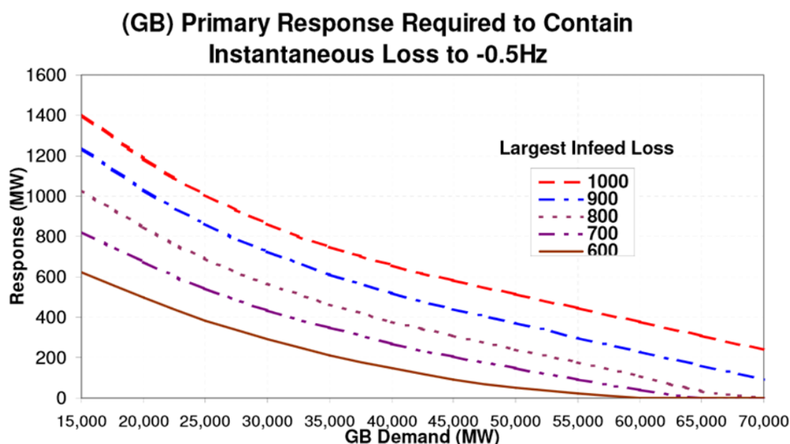
Figure 4.4 – Primary response in Great Britain market as function of demand and contingency size
