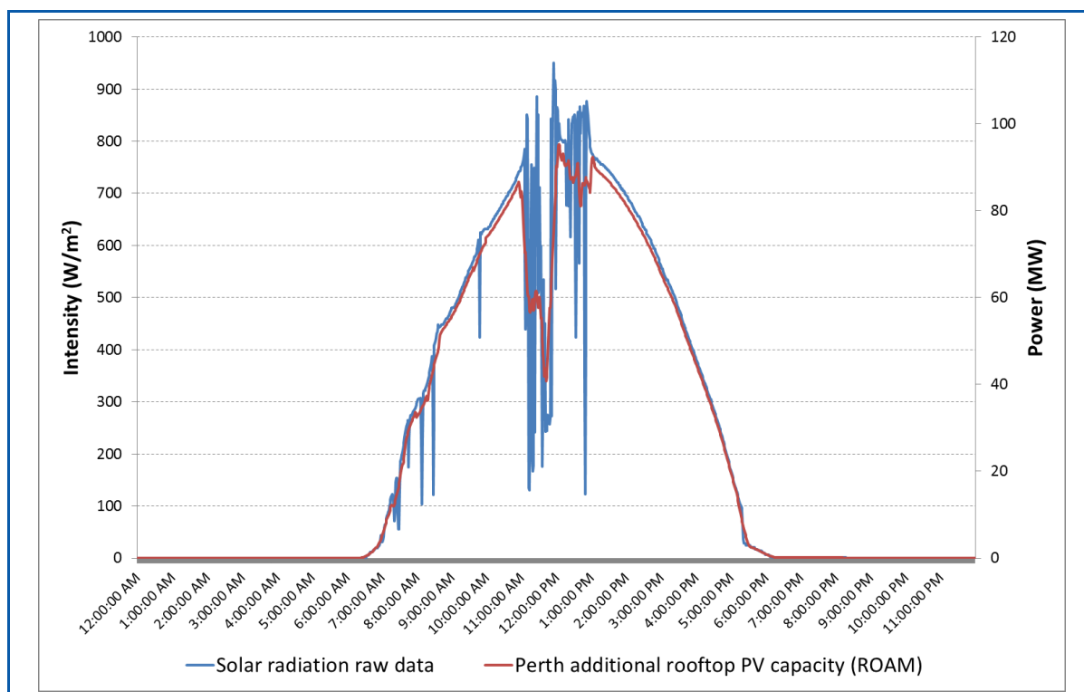
Figure A.1 – The System Management control centre's solar radiation data and ROAM's derived rooftop PV trace for Perth for 3 April 2013
