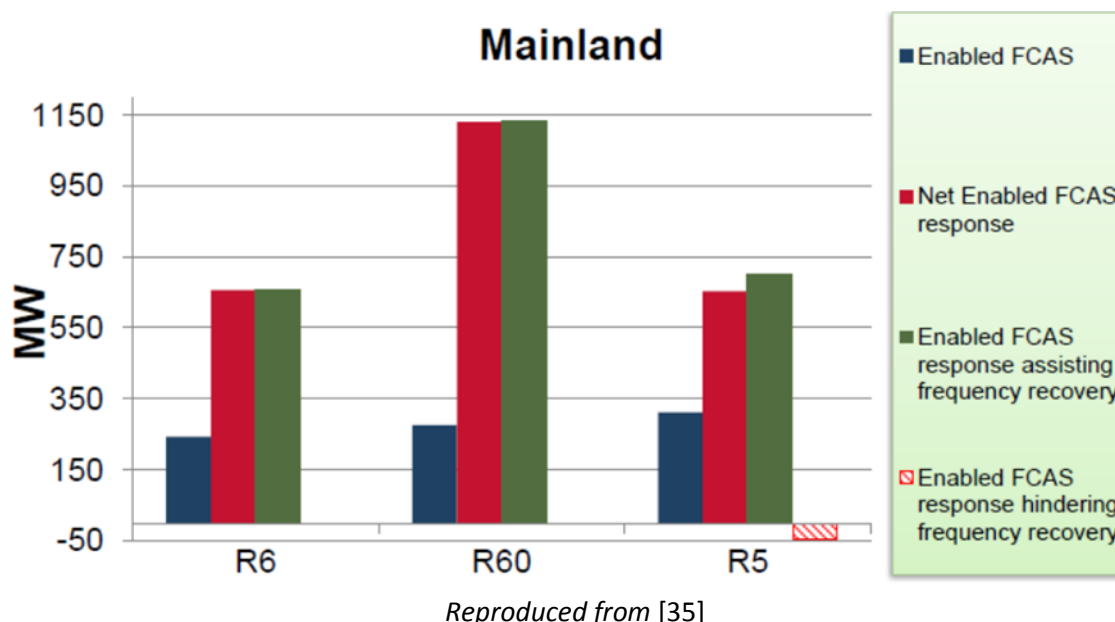
Figure 6.3 – Available FCAS capacity in the mainland NEM in response to a multiple contingency event.
