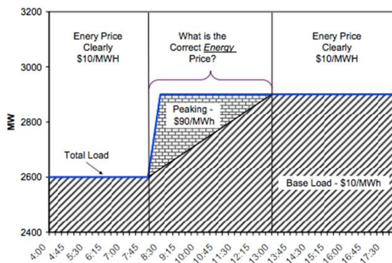
Figure 6.2 – Possible situation requiring ramping market
