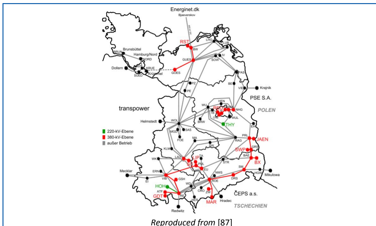
Figure 12.5 – 50Hertz grid SRAS providers and re-energization paths
