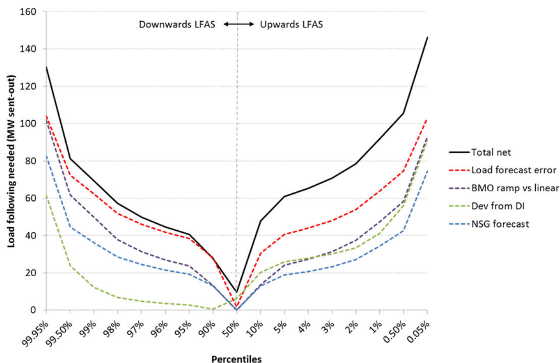
Figure 9.1 – ROAM percentile estimates for LFAS needed based on the full year of data
