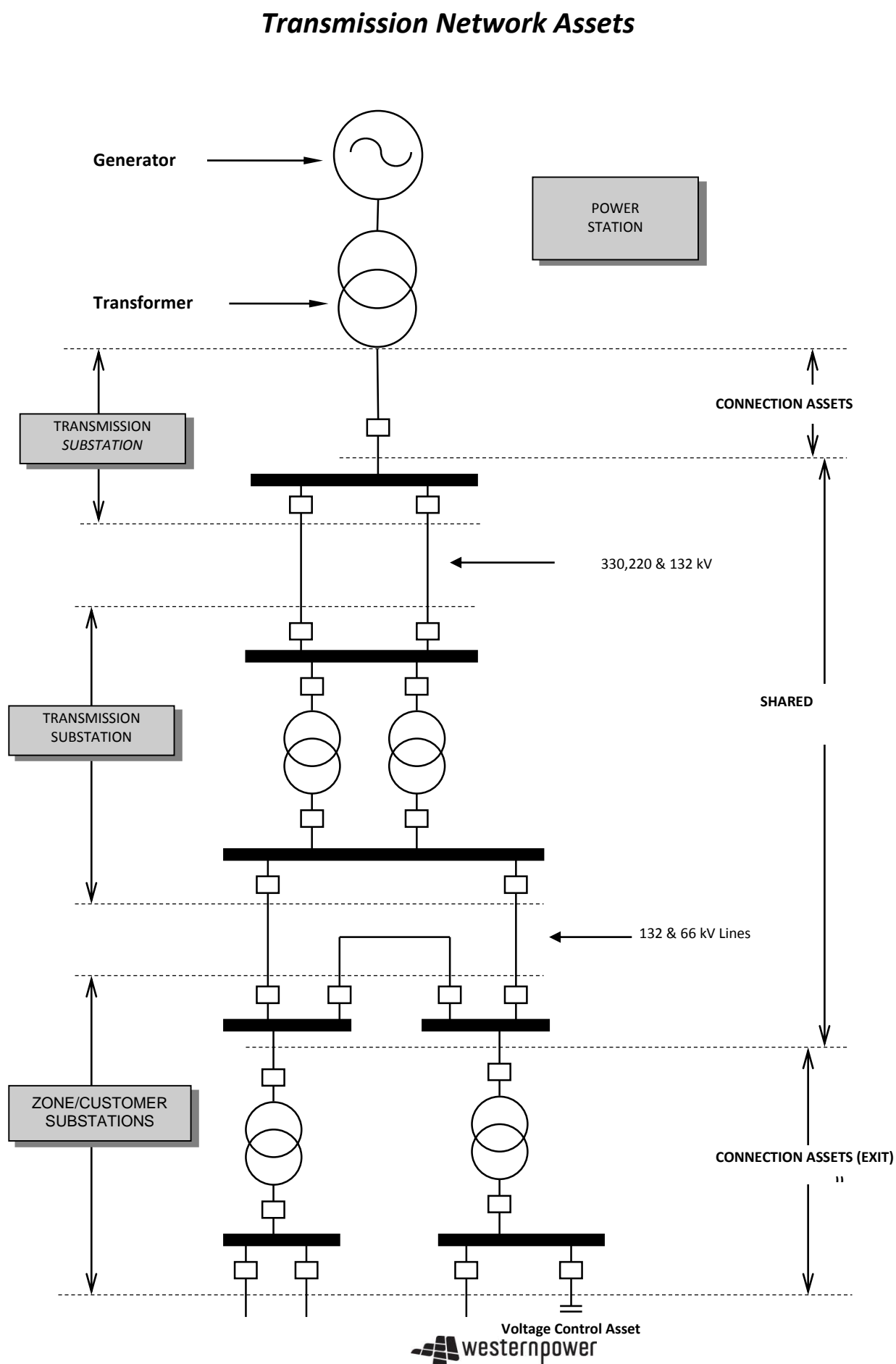
Figure 2 - Transmission Network Assets
