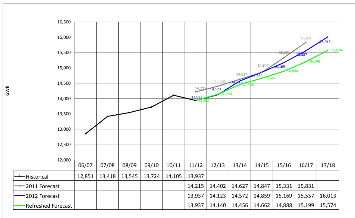
Figure 1 Distribution energy consumption history and forecasts (GWh)
