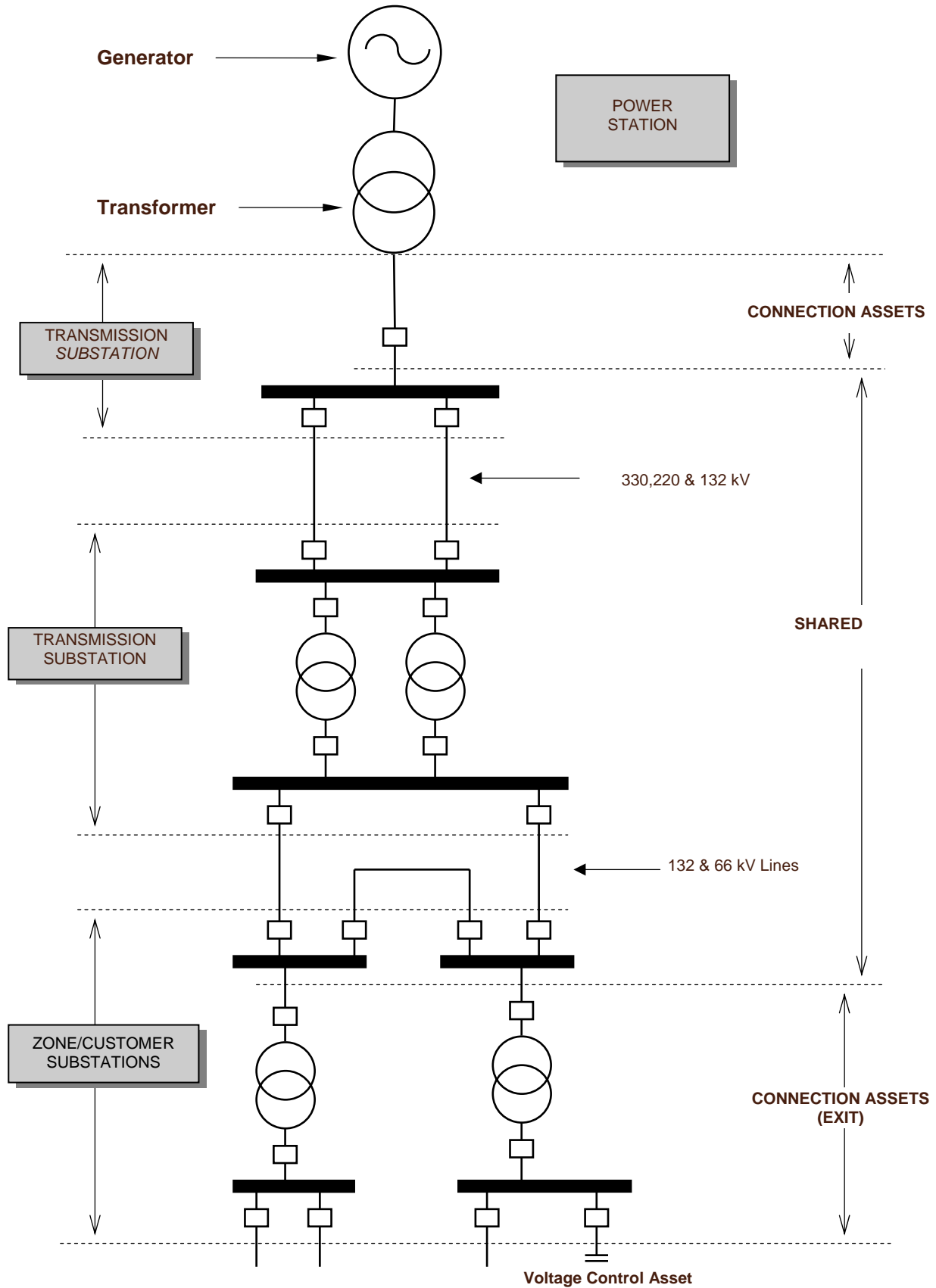
Figure 2 - Transmission Network Assets
