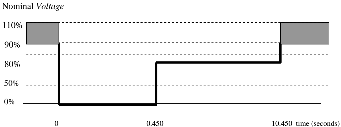
Figure 3.5 – Off nominal voltage operation capability requirement for generating units .
