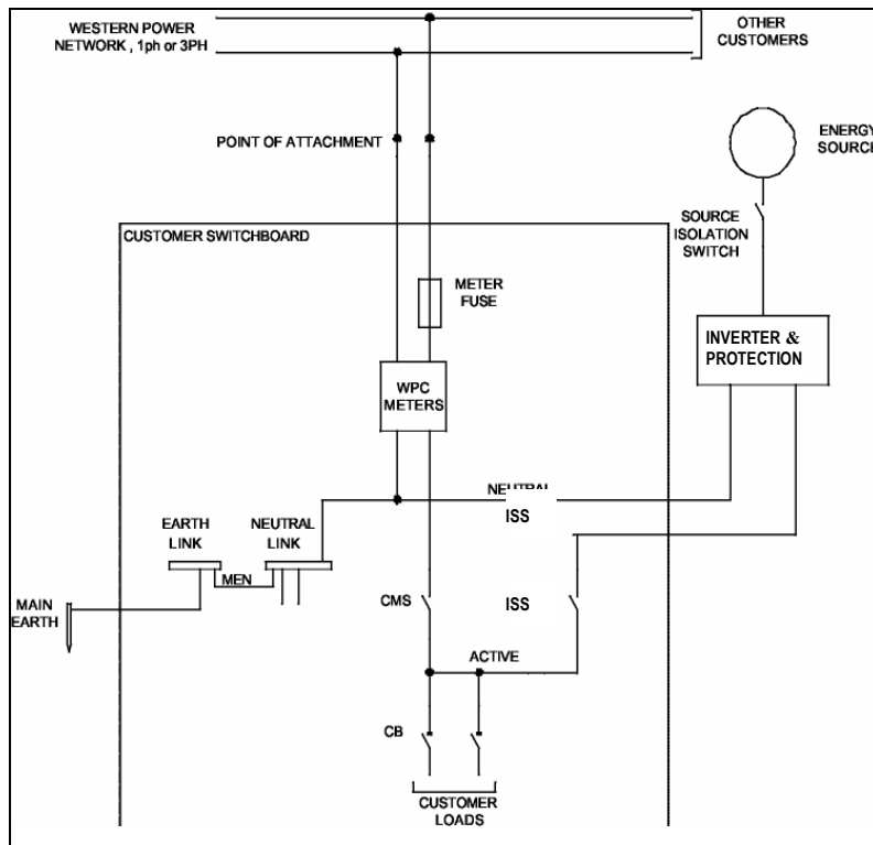
Figure 3.7 Schematic diagram for the connection of an inverter energy system
