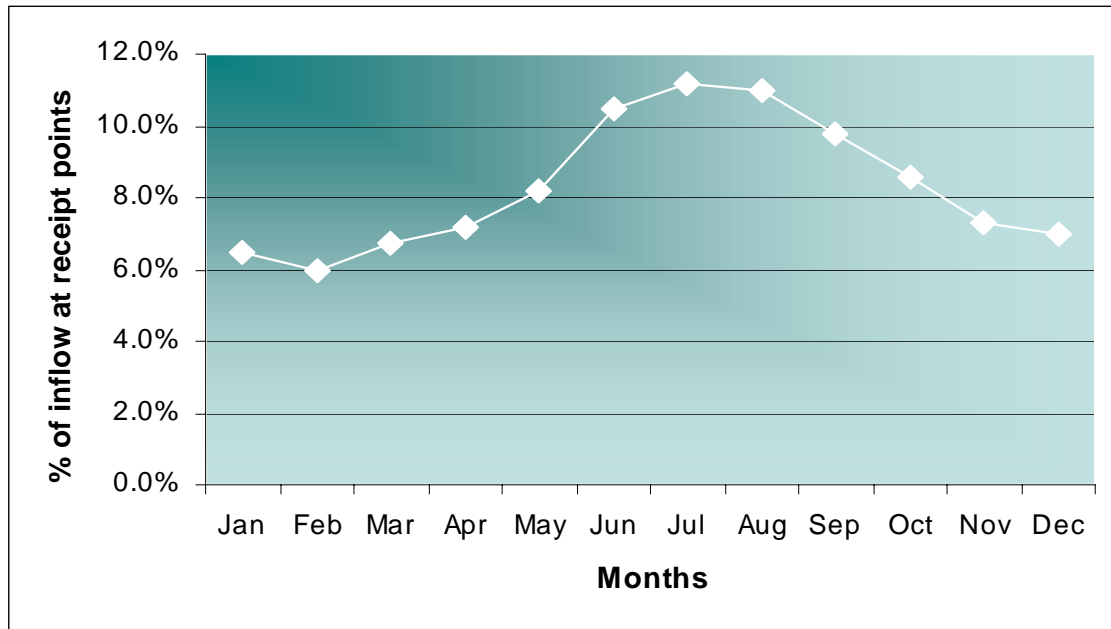
FIGURE 6.1 - SYSTEM LOAD PROFILE BY MONTH
